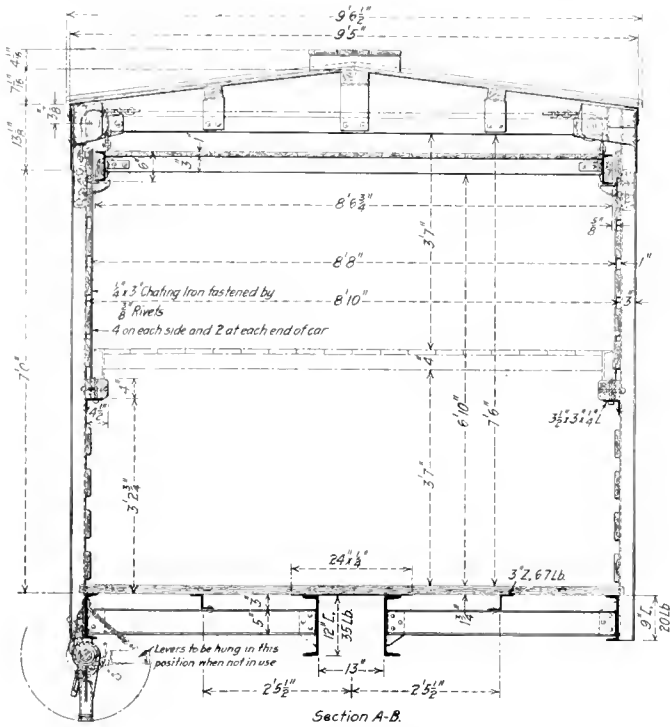
Cross Section Showing the Deck Operating Mechanism
